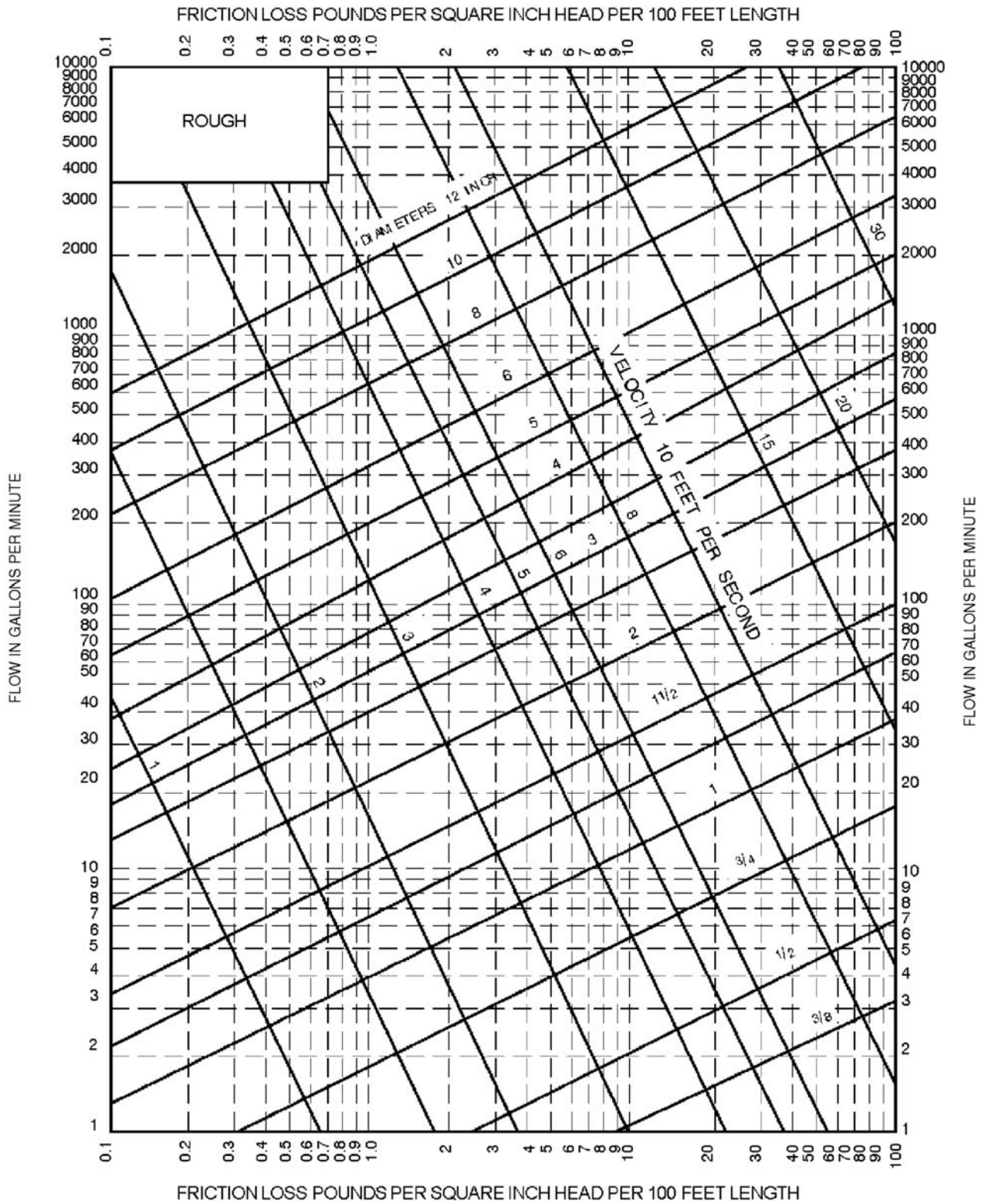
FIGURE AP103.3(7) FRICITION LOSS IN FAIRLY ROUGH PIPE a
